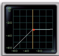
Hard knee
